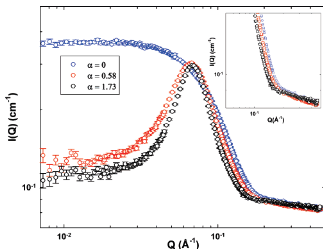
Figure 3. Comparison of the SANS scattering intensities of PAMAM dendrimers of generation 4 in D 2 O solutions with concentration of 0.0225 g/mL obtained at \alpha = 0 , 0.58, and 1.73 respectively. The enlarged high- Q parts of the scattering intensities are given in the inset.
