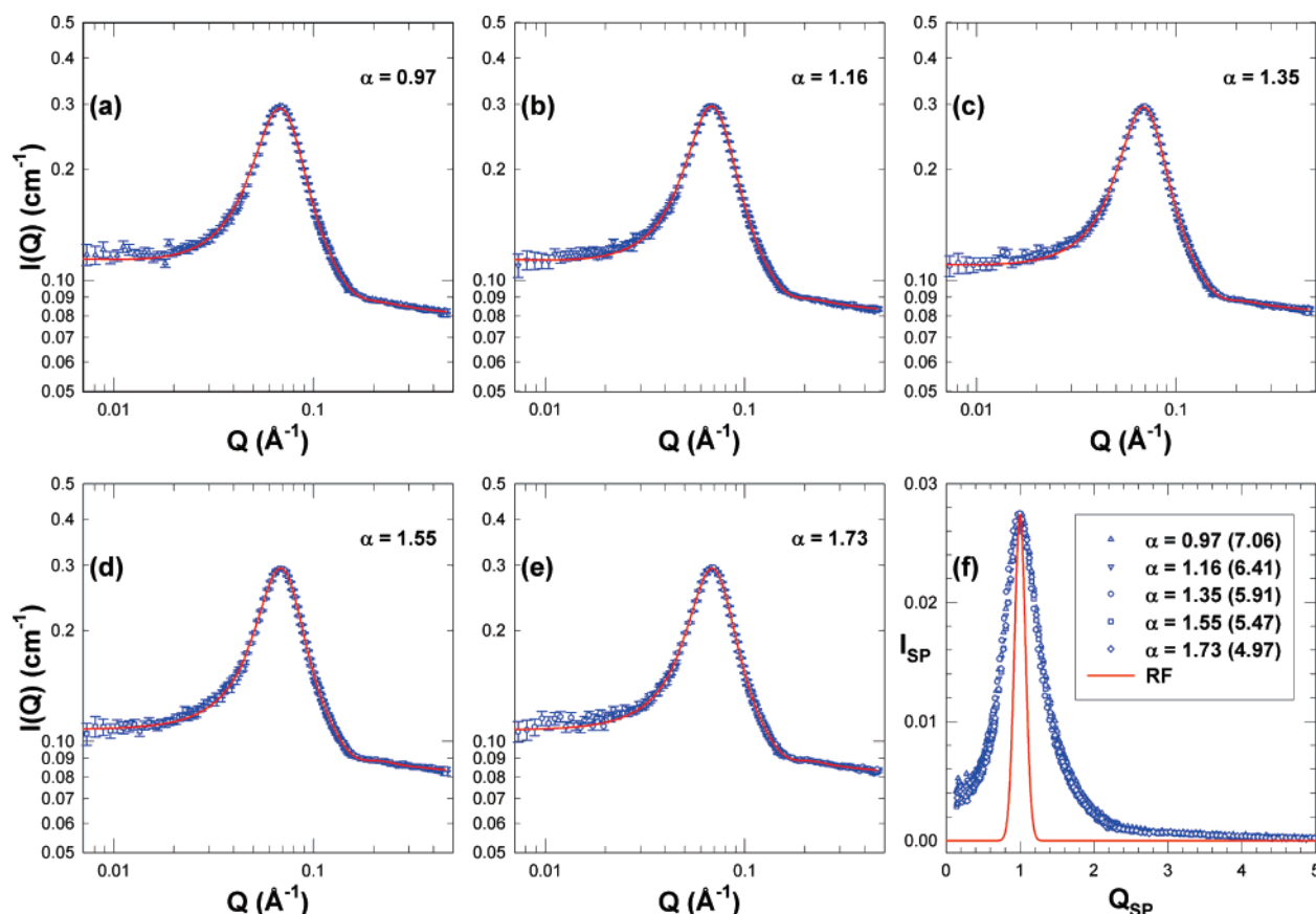
Figure 5. Same as Figure 3 but in a different \alpha range. Unlike the previous Figure, within this \alpha range ( 0.97 < \alpha < 1.73 , 7.06 > pD > 4.97 ), all the SANS intensity distributions are essentially identical to each other. It can be clearly seen from panel f that the local order and the inter-dendrimer interaction in solutions remain unchanged even with the progressive increment of the deuteron concentration in the solution and the degree of dendrimer molecular protonation. It can also be noticed that all the scaled curves are significantly broader than the resolution function of the NG3 spectrometer, indicating that the great similarity of the SANS intensity distributions is not resolution limited.
